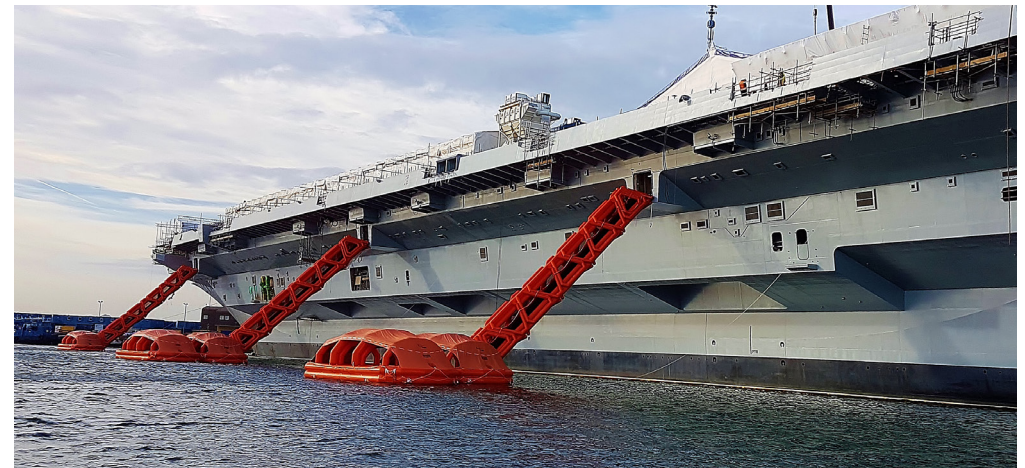
Liferaft Systems Australia Marine Evacuation System installed on the Royal Navy's (UK) Queen Elizabeth class aircraft carriers
